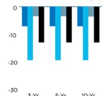
Maximum Drawdown (%)
