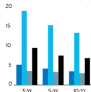
Standard Deviation (%)
